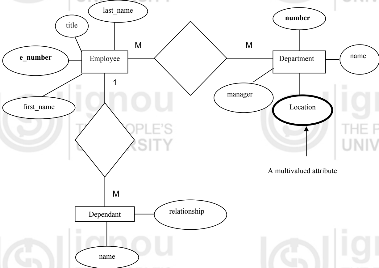
Figure 9.13: E-R Diagram for Employee database
