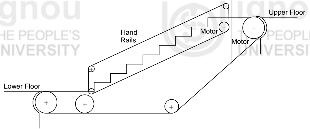
Figure 8.2 : Escalator
