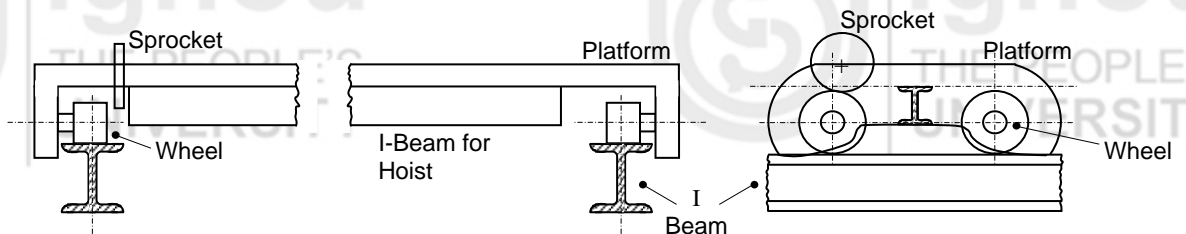
Figure 8.9 : An Overhead Crane
