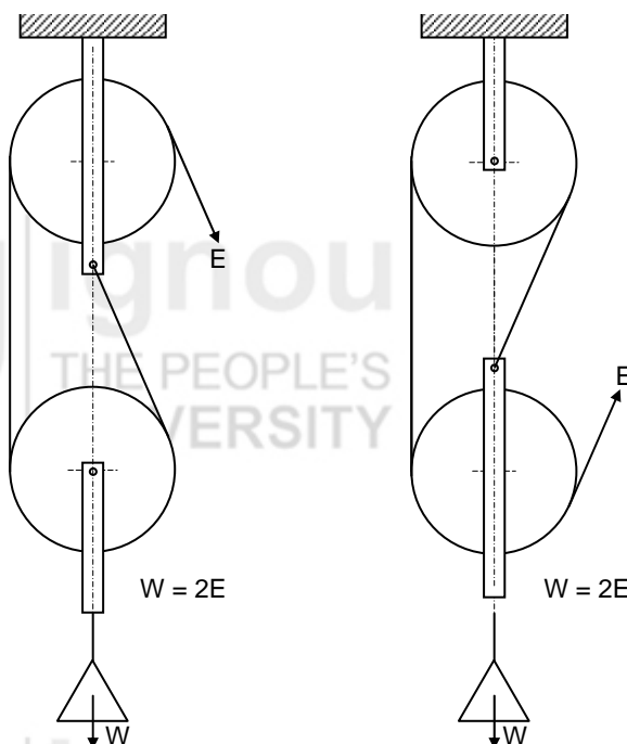
Figure 8.4 : Pulley Arrangement for Portable Hoists
